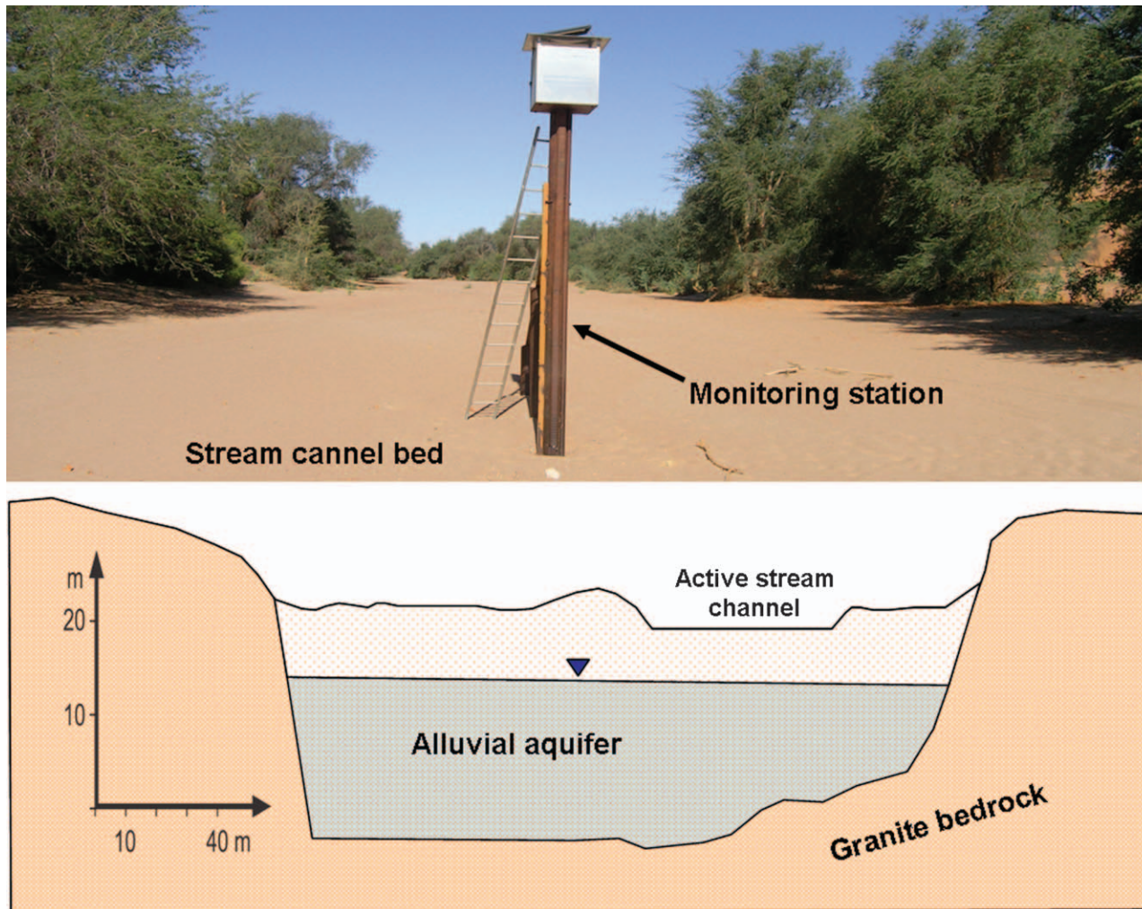
Figure 2. The Kuisieb River stream channel and the monitoring station by the Gobabeb research centre (above) and a typical lithological cross section of the Kuisieb River aquifer at the study area (below).
