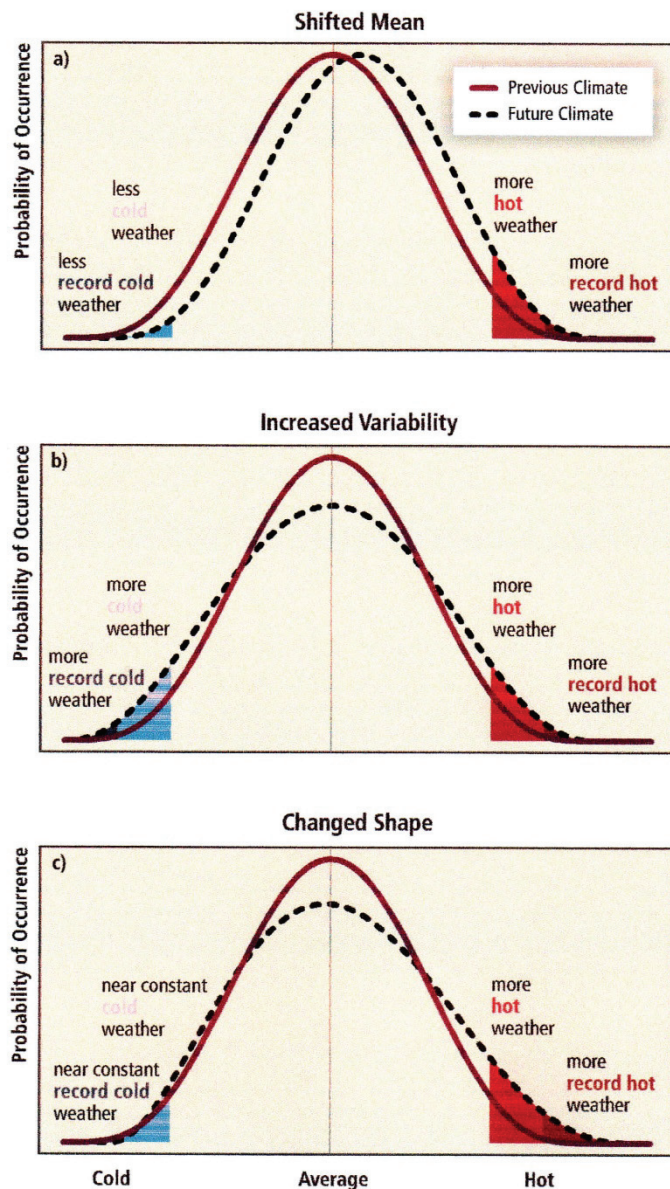
Figure 2.1. The effect of changes in temperature distribution on extremes. Different changes in temperature distributions between present and future climate and their effects on extreme values of the distributions: a) effects of a simple shift of the entire distribution toward a warmer climate; b) effects of an increased temperature variability with no shift of the mean; and c) effects of an altered shape of the distribution, in this example an increased asymmetry toward the hotter part of the distribution.
