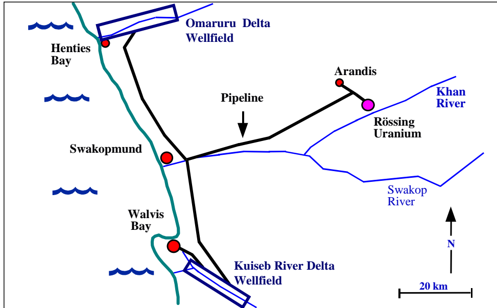
Figure 2: Central Namib Water Supply Scheme
