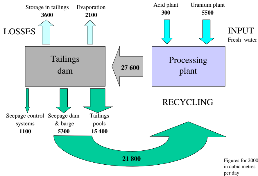
Figure 3: Rössing Uranium Process Water Circuit
