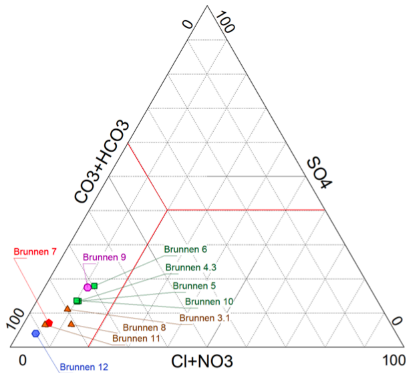
Diagram 4.1.2 The proportions of anion in the water
