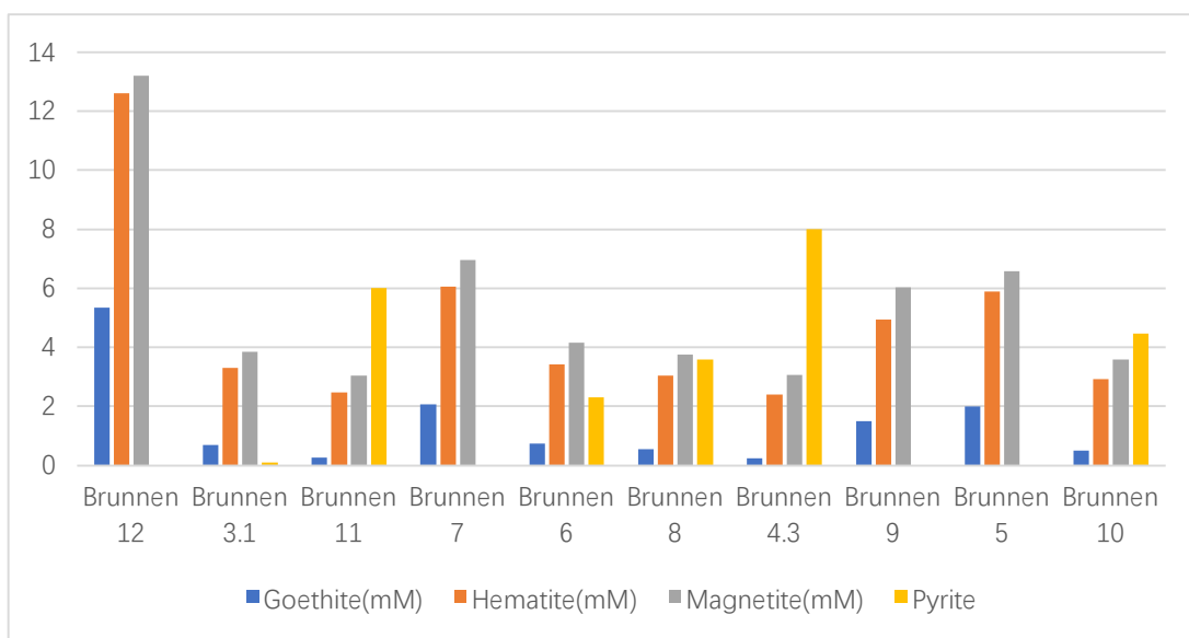
Diagram 4.3.2 presipitation of Goethite, Hematite, Magnetite, Pyrite analyzed by Aqion
