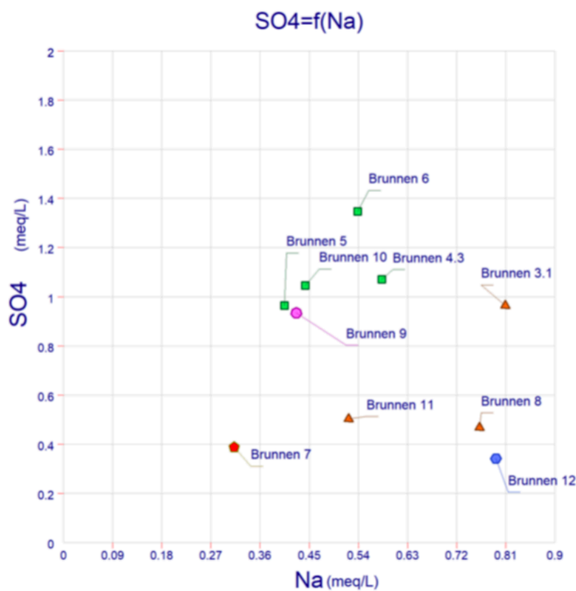
diagram 4.2.3 relationship of Na and \text{SO}_4
