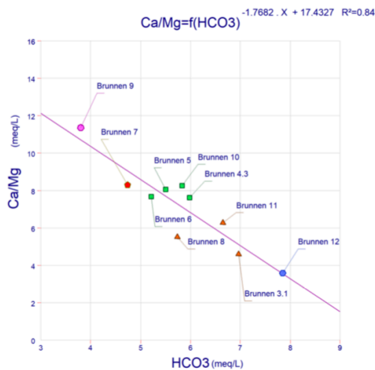
diagram 4.2.2 relationship of Ca/Mg and HCO 3 -
