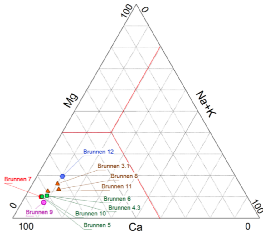
Diagram 4.1.1 The proportions of Cation in the water
