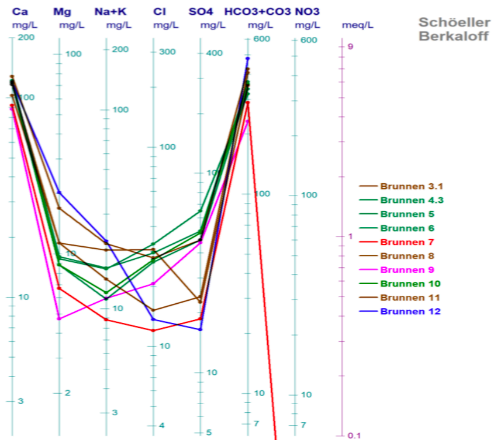
Diagram 4.1.3 Cations and anions analysis by Schoeller Diagramm
