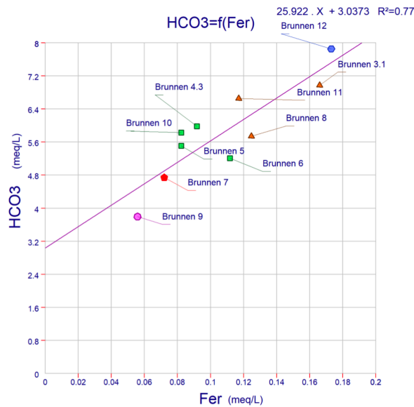
diagram 4.2.1 relationship of Fe and HCO 3 -
